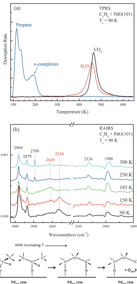
Figure 2. a) TPRS traces of propane, H 2 O and CO 2 obtained after saturating a PdO(101) film with undeuterated propane at 90 K. b) Series of RAIRS spectra obtained after heating a saturated propane layer on PdO(101) to the temperatures indicated. Each RAIRS spectrum was obtained using a freshly prepared PdO(101) film and the frequencies of softened C–H stretch bands are labeled in red. c) Schematic illustration showing the evolution of adsorbed configurations of propane on PdO(101) during TPRS.
